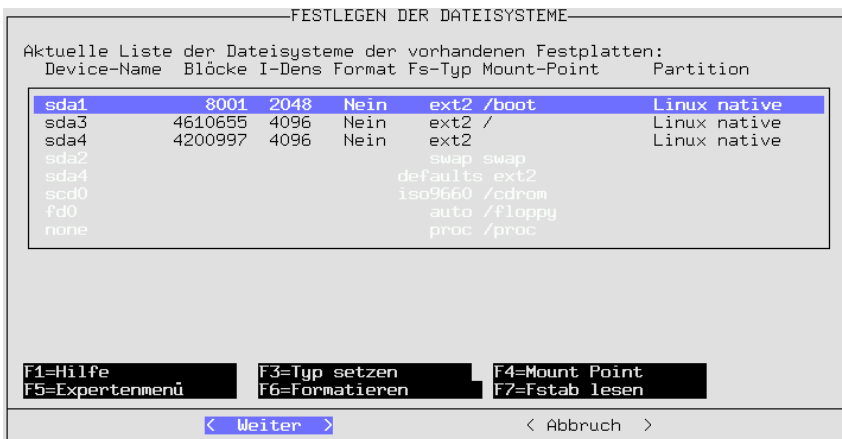
Abbildung 3.14: YaST – Mountpoints
