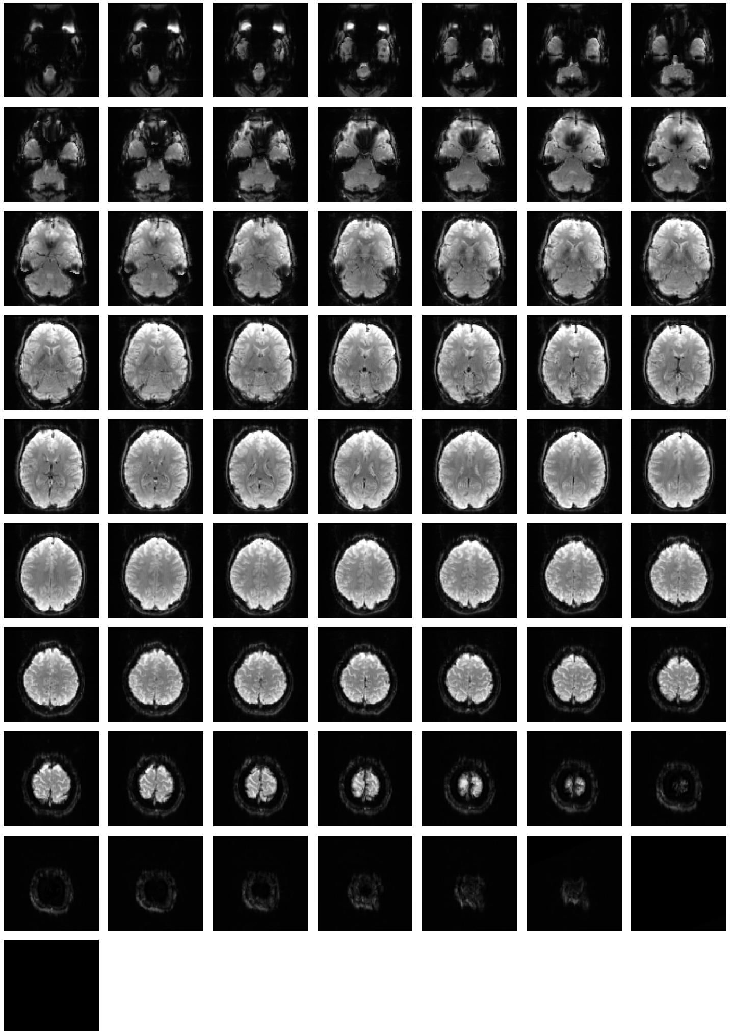
Mean EPI
