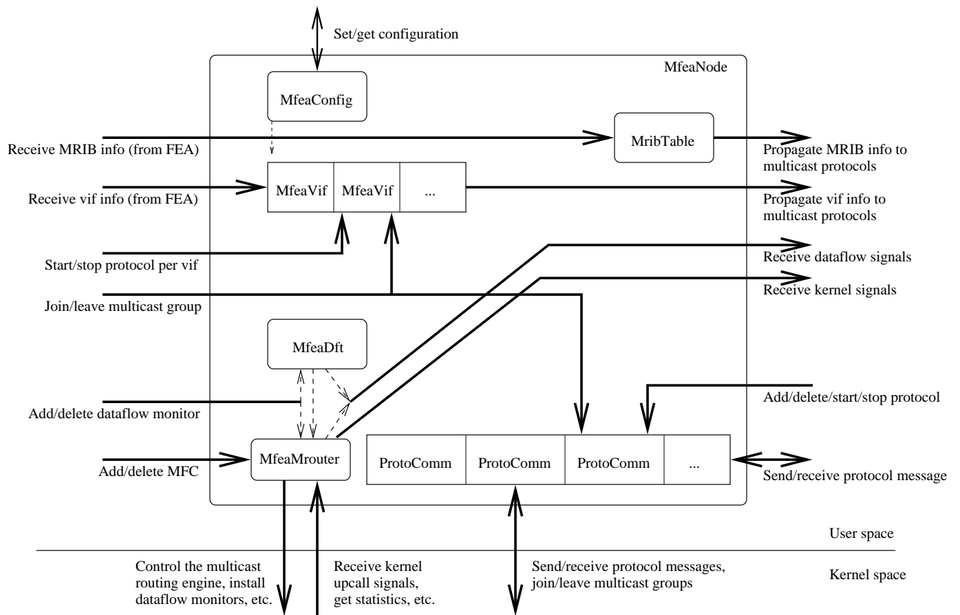
Figure 1: MFEA design overview
