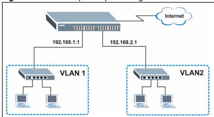
Figure 28 Initial Setup Example: Management IP Address
