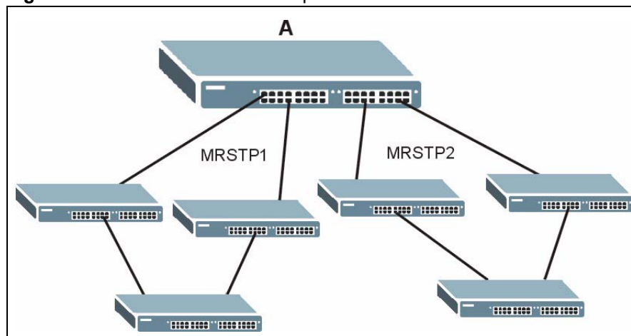
Figure 54 MRSTP Network Example
