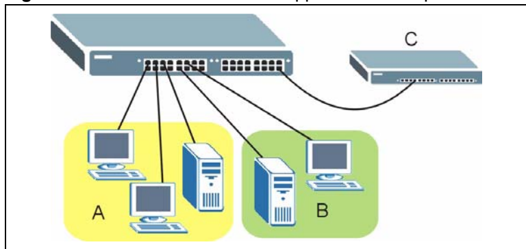
Figure 47 Protocol Based VLAN Application Example
