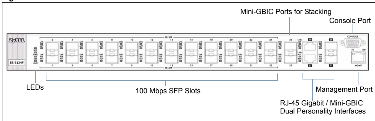
Figure 12 Front Panel: ES-3124F
