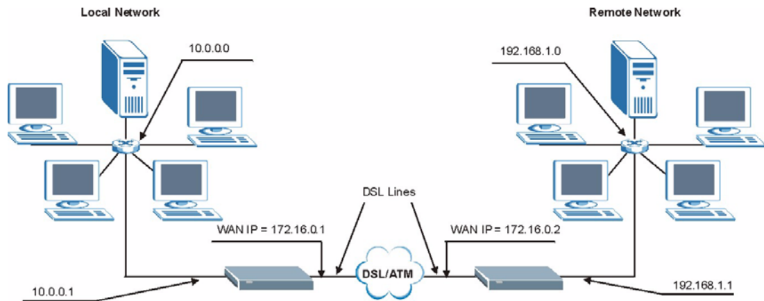
Figure 75 Sample IP Addresses for a TCP/IP LAN-to-LAN Connection
