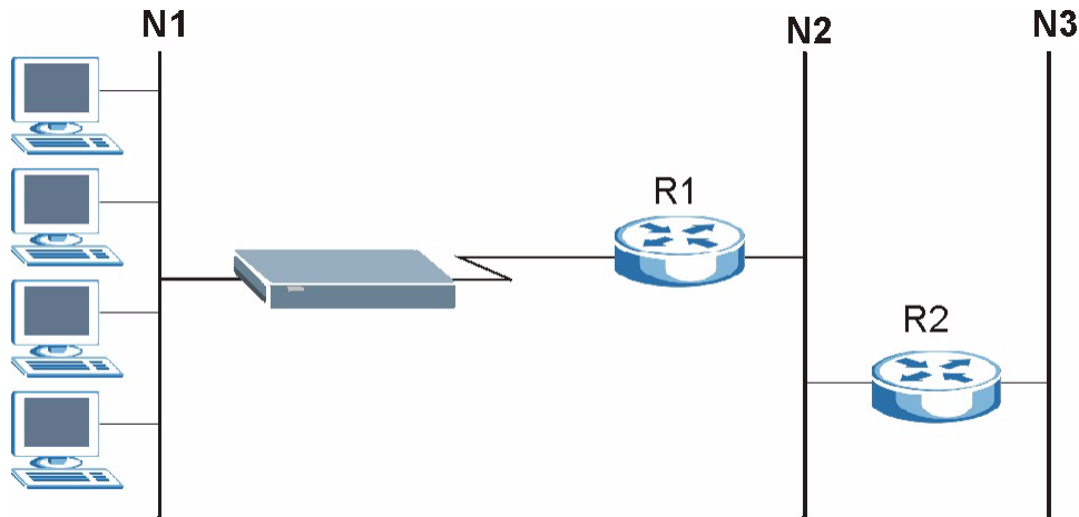
Figure 86 Sample Static Routing Topology
