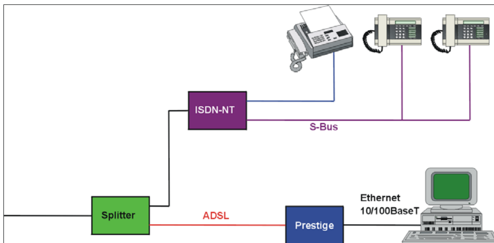
Figure 199 Prestige with ISDN
